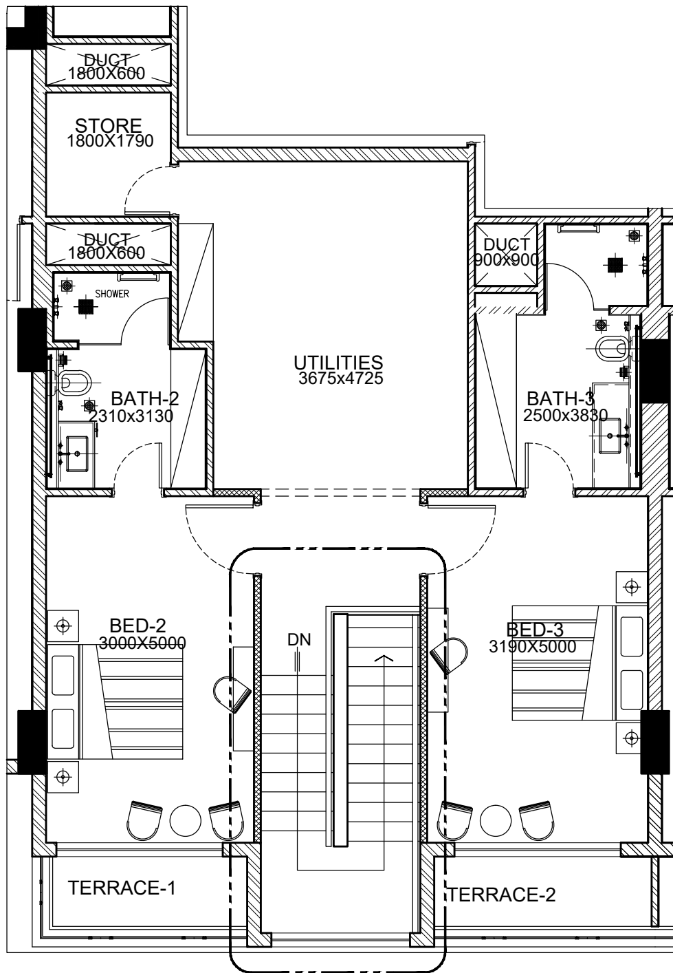
2 AD-101-22 TYPE 3-C UPPER LEVEL LAYOUT PLAN SCALE 1:75
