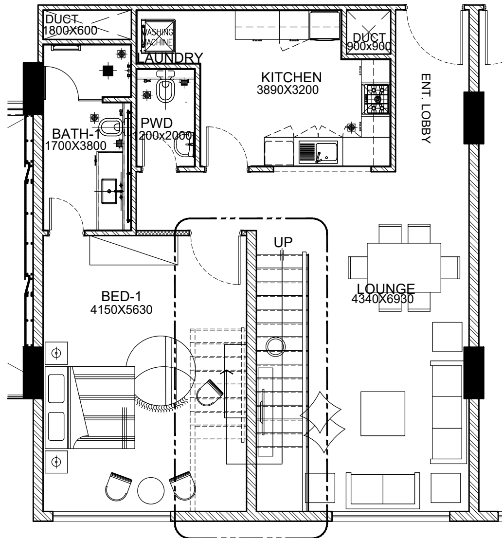
1 AD-101-20 TYPE 3-B LAYOUT PLAN SCALE 1:75
