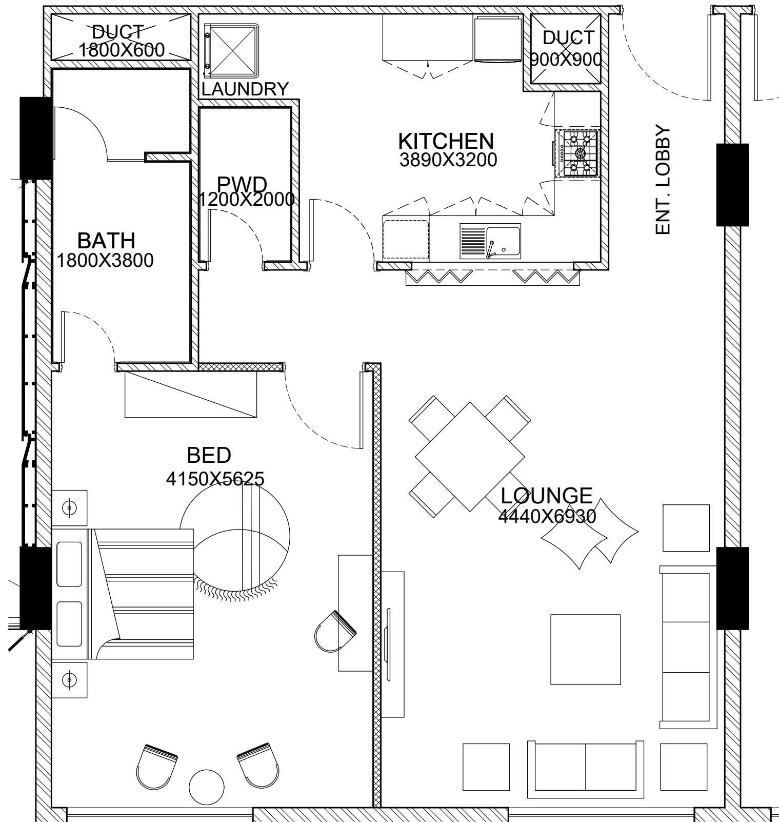
1 AD-101-15 TYPE 1-B LAYOUT PLAN SCALE 1:50
