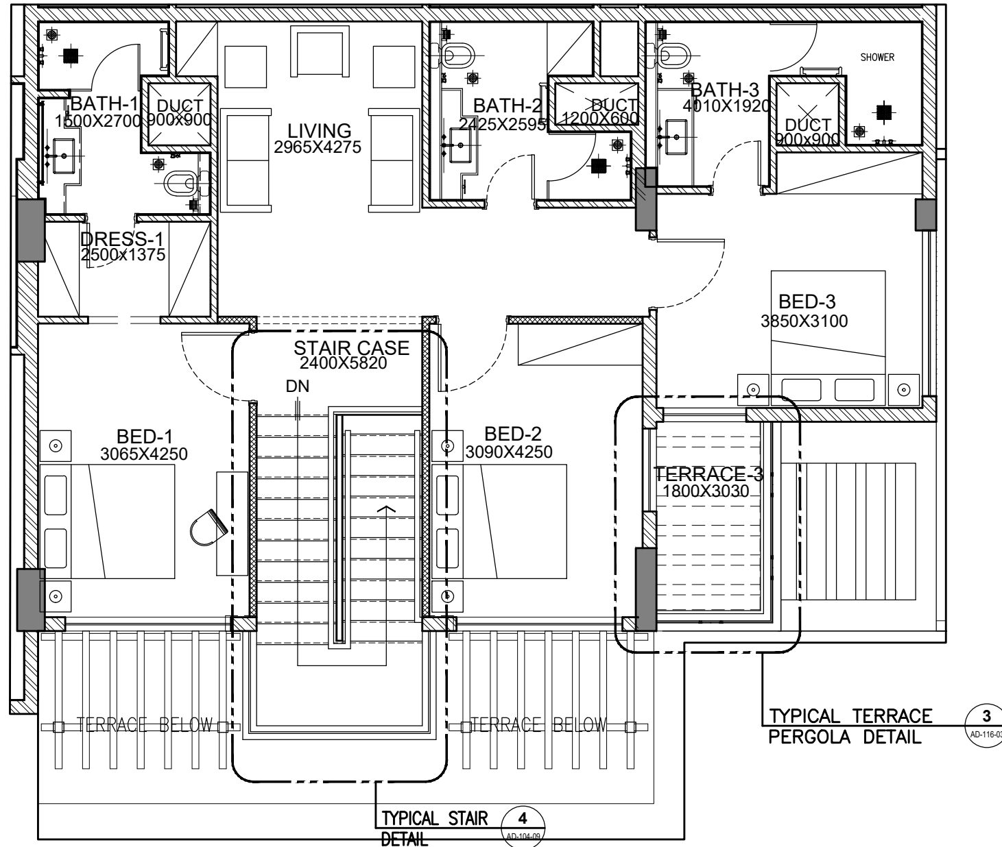
2 AD-101-21 TYPE 3-E UPPER LEVEL LAYOUT PLAN SCALE 1:75
